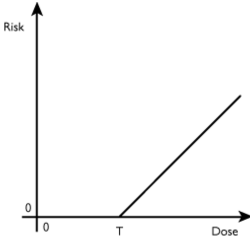
Figure 3: Threshold Hypothesis
