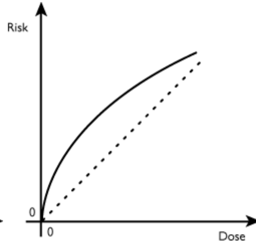
Figure 4: Supralinear Hypothesis
